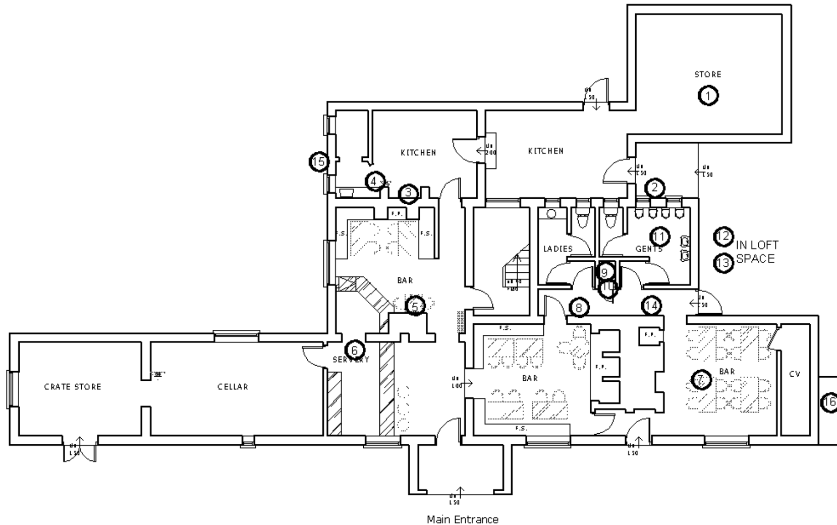
Description of Drawing: Site layout
