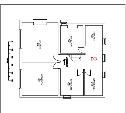
Plan of First Floor 1:100
